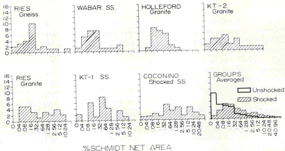
Fig. 13. Histograms which indicate some basic differences in distribution of areas of optic axis dispersal polygons of quartz crystals from both unshocked and shocked rocks. The size classes, in terms of percent of Schmidt net area, start with 0.04 to absorb basic errors of measurement. The averaged histograms in the last diagram emphasize the differences and show the smoothing to be expected from measuring a larger number of grains.
